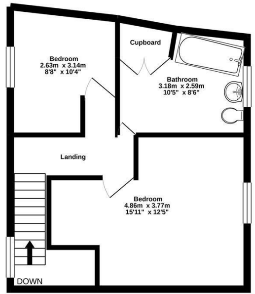
1ST FLOOR 38.0 sq.m. (410 sq.ft.) approx.
