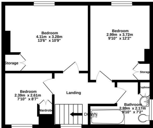
1ST FLOOR 41.0 sq.m. (442 sq.ft.) approx.
