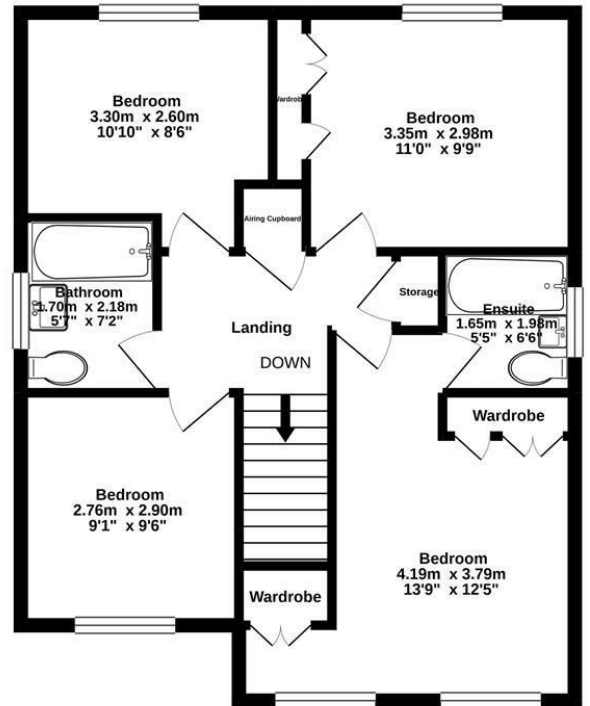
1ST FLOOR 56.7 sq.m. (611 sq.ft.) approx.
